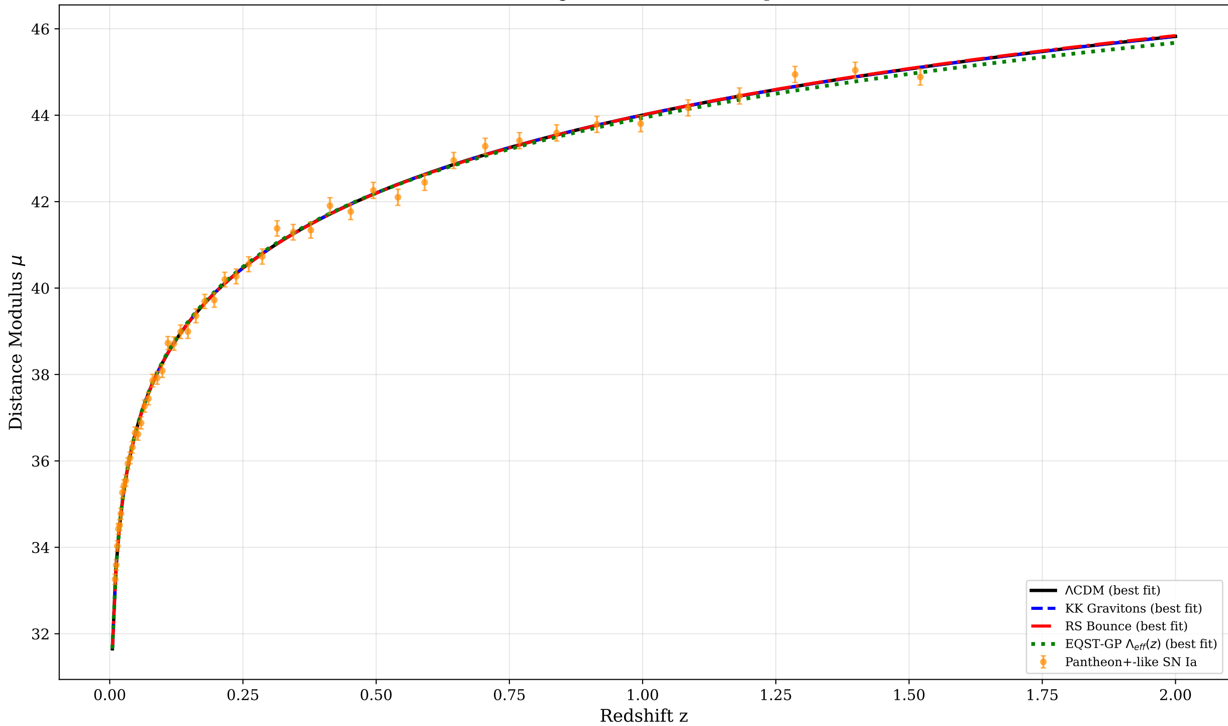
Hubble Diagram: Four-Model Comparison
