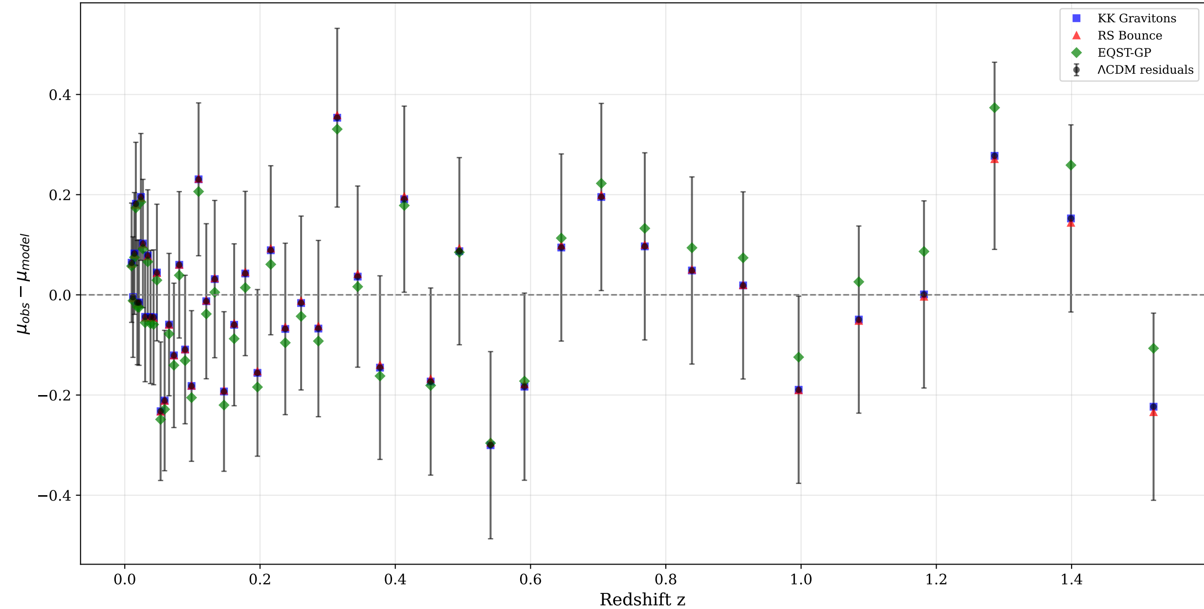
Hubble Diagram Residuals
