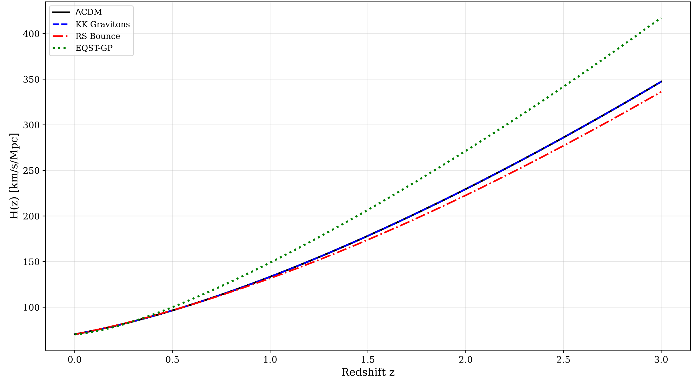
Expansion Rate H(z) : Model Comparison
