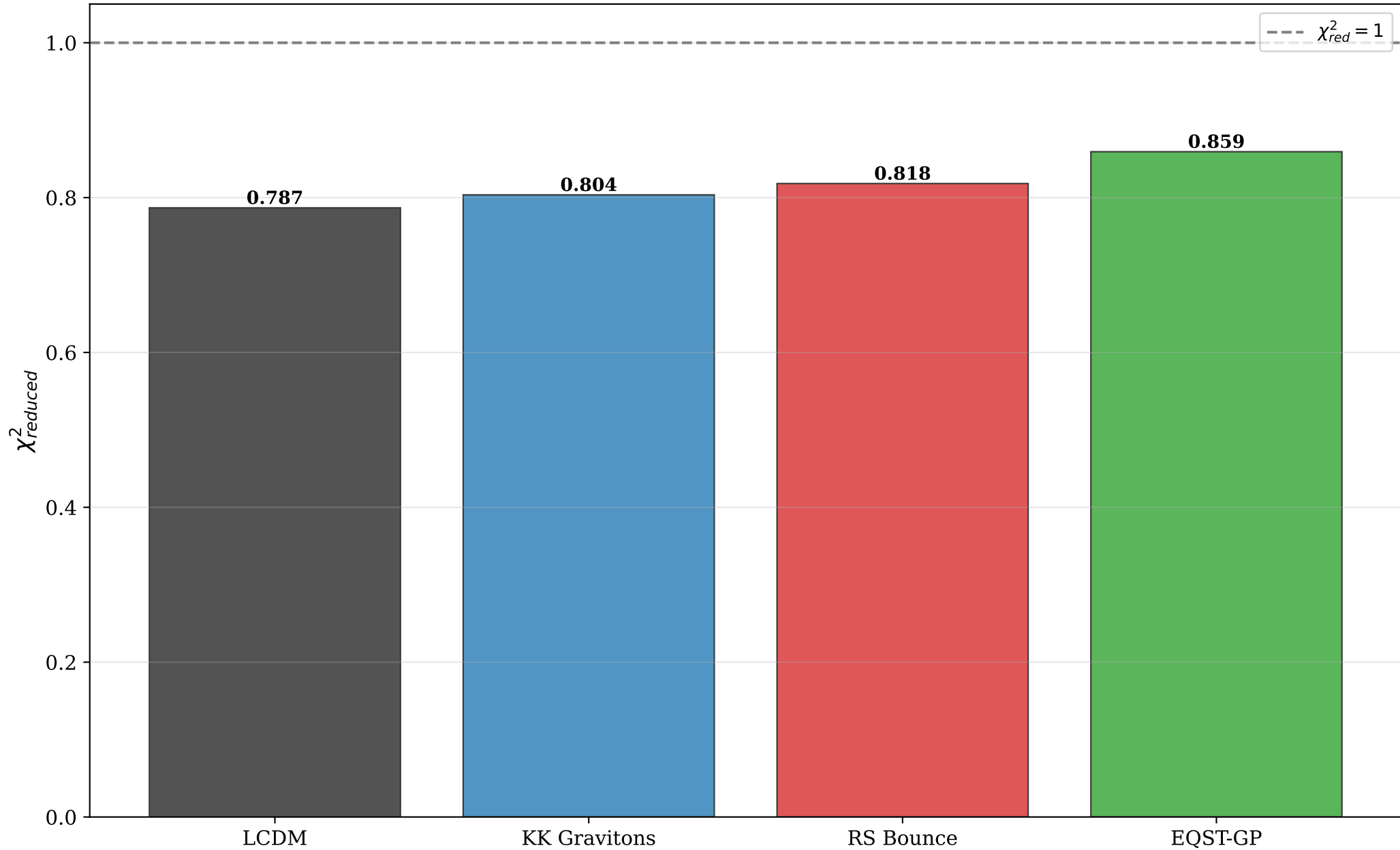
Goodness-of-Fit: Model Comparison (SN Ia)
