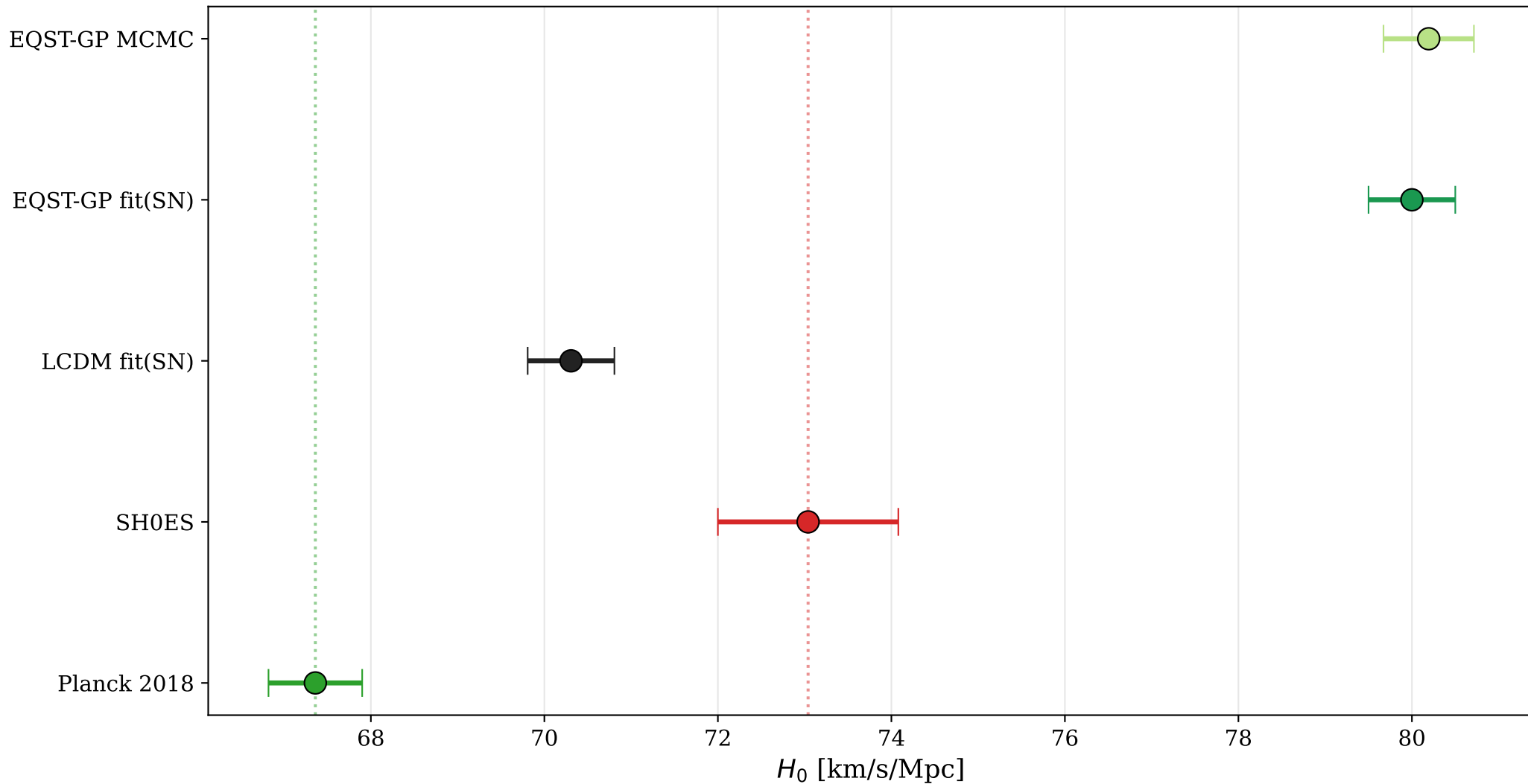
Hubble Constant: Cross-Method Comparison and Tension
