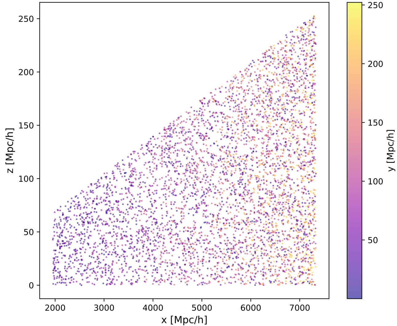
Galaxy Distribution (x-z plane)
