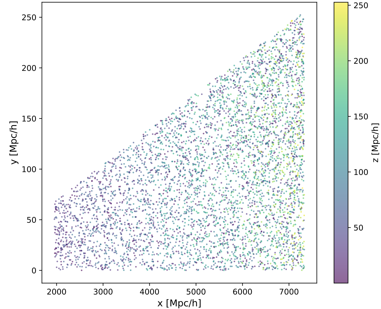
Galaxy Distribution (x-y plane)
