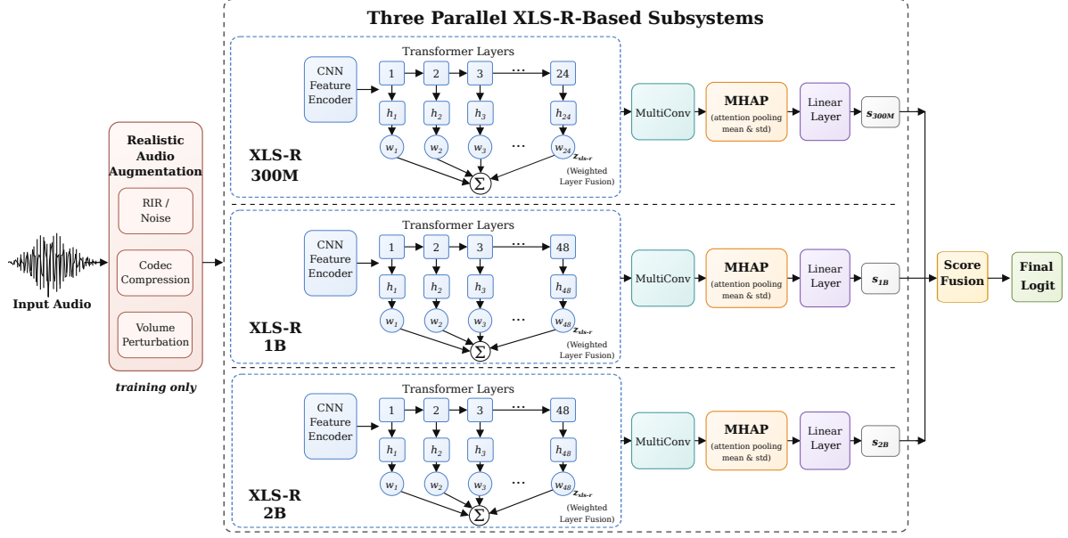
Figure 1: Overview of the proposed system. Realistic audio augmentation simulates environmental and transmission degradations during training. Each subsystem uses an XLS-R front end with learnable layer-wise weighted fusion, followed by a MultiConv–MHAP back end. The scores of the three subsystems are fused to produce the final logit.
