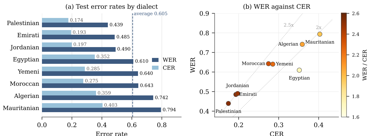
Figure 1: (a) Final test WER and CER per dialect, ordered by WER; the dashed line marks the country-average WER of 0.6053. (b) WER against CER, colored by their ratio, with dotted lines at ratios of 2.0 and 2.5. Dialects near the 2.5 line lose many words to small character differences, which is the pattern the canonicalization step targets. Egyptian is the clear outlier at 1.7.
