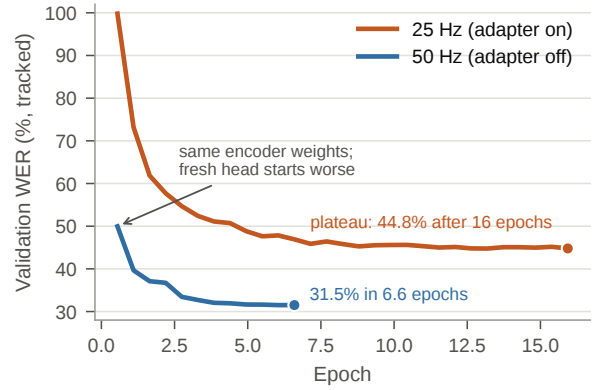
Figure 2: Subtask 1.3 validation trajectories. The 25 Hz run trains from the pretrained encoder with the adapter enabled. The 50 Hz run resumes from the encoder weights of that run at its 16-epoch plateau, with the adapter disabled and a newly initialized CTC head, on the same data and schedule; its epoch axis counts epochs after the restart. The fresh head starts above the 44.8% plateau it resumes from and crosses below it within two epochs.
