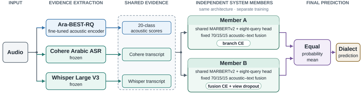
Figure 1: Task 2 final inference pipeline. Acoustic evidence is combined with independently generated Cohere and Whisper transcripts. Two separately trained eight-query members share the architecture but use different objectives; their probability distributions are averaged.
