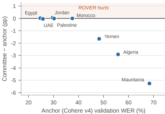
Figure 3: Subtask 1.1 development data: WER of the final routed committee minus WER of the Cohere v4 anchor alone, against the anchor’s country-specific development WER. Cohere v4 trained on this development split, so the anchor WERs are in-domain and the differences are those seen during committee selection.
