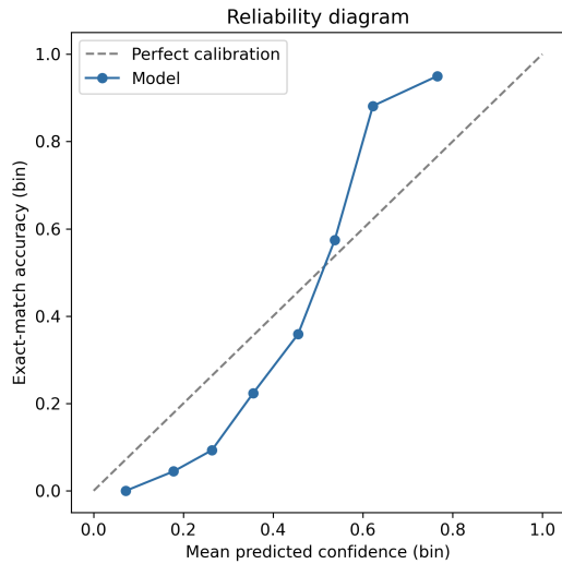
Figure 3: Reliability diagram: mean predicted confidence vs. exact-match accuracy per bin, Development set.
