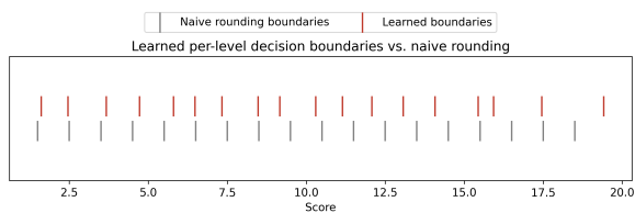
Figure 4: Learned per-level decision boundaries (Section 3.6) compared to naive integer-rounding thresholds, Development set.
