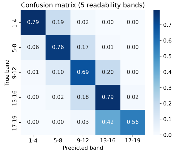
Figure 2: Confusion matrix grouped into five readability bands.
