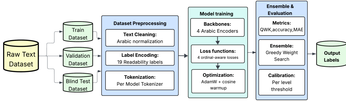
Figure 1: End-to-end pipeline of the heterogeneous 7-model ensemble for fine-grained Arabic readability assessment
