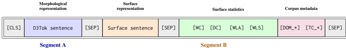
Figure 1: Structure of the combined model input. Segment A contains the D3Tok morphological representation. Segment B contains the normalized surface sentence, surface statistics, and corpus metadata. Special tokens delimit the individual components.
