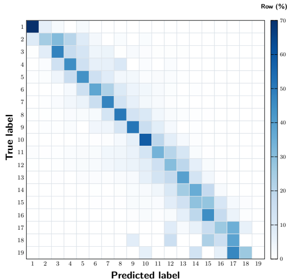
Figure 2: Confusion matrix on the development set.
