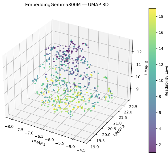
Figure 14: Three-dimensional UMAP projection of EmbeddingGemma-300M sentence representations, colored by readability class.
