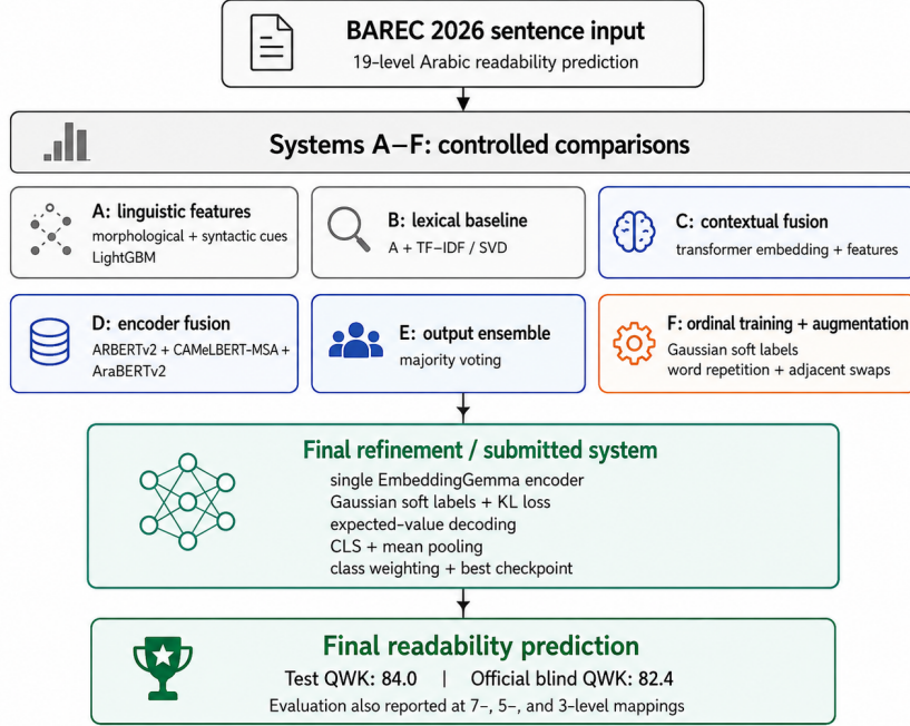
Figure 1: Overview of the BAREC 2026 system progression. Systems A–F provide controlled comparisons from linguistic and lexical baselines to contextual, multi-encoder, ensemble, and ordinal-aware configurations.
