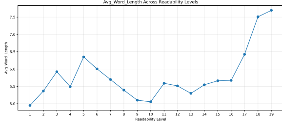
Figure 3: Average word length across readability classes.
