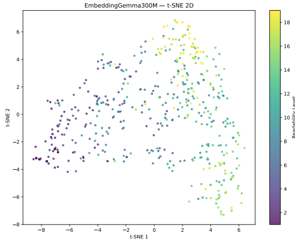
Figure 13: Two-dimensional t-SNE projection of EmbeddingGemma-300M sentence representations, colored by readability class.
