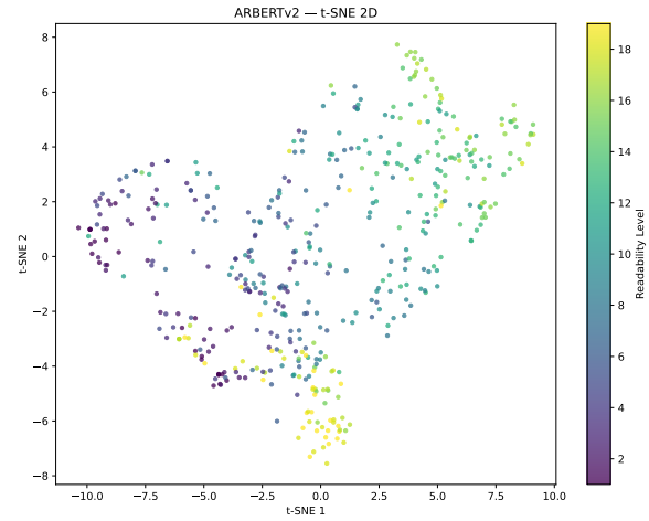
Figure 9: Two-dimensional t-SNE projection of ARBERTv2 sentence representations, colored by readability class.
