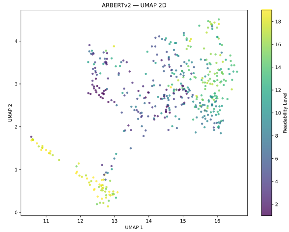
Figure 8: Two-dimensional UMAP projection of ARBERTv2 sentence representations, colored by readability class.
