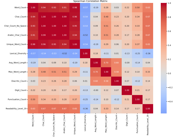
Figure 5: Spearman correlation matrix of the extracted linguistic features.
