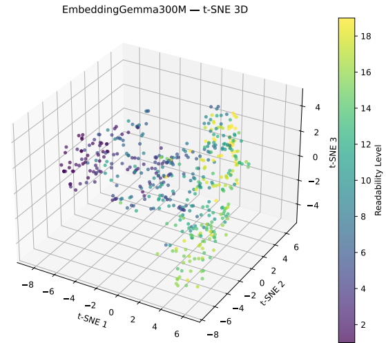
Figure 15: Three-dimensional t-SNE projection of EmbeddingGemma-300M sentence representations, colored by readability class.
