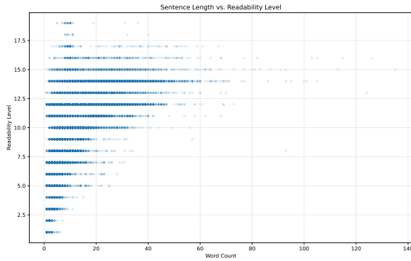
Figure 7: Relationship between sentence length and readability level.
