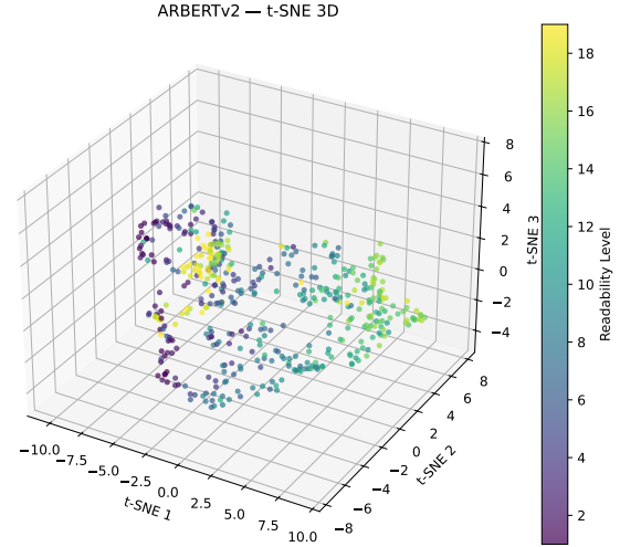
Figure 11: Three-dimensional t-SNE projection of ARBERTv2 sentence representations, colored by readability class.
