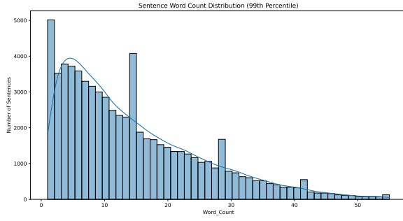
Figure 6: Distribution of the number of words per sentence across readability classes.
