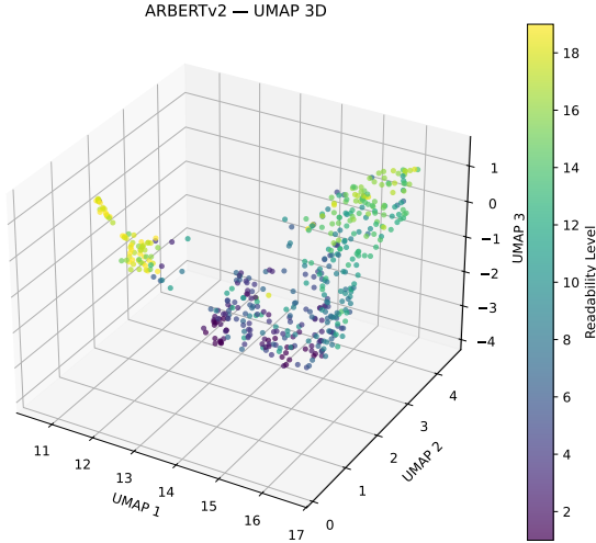
Figure 10: Three-dimensional UMAP projection of ARBERTv2 sentence representations, colored by readability class.
