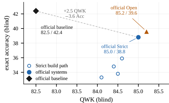
Figure 2: Exact accuracy vs. QWK on the blind set: the Strict build path (hollow), the two official systems (filled), and the official baseline, which sits 2.5 QWK below official Strict at 3.6 higher exact accuracy. The metrics reward different prediction styles.
