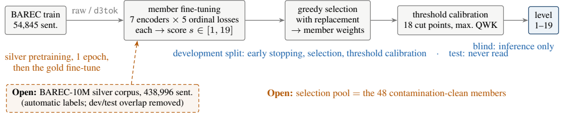
Figure 1: Both systems and what is fitted where: the shared pipeline (gray) trains on the training split, blue states the role of every other split, and orange (dashed) marks the two Open-track additions.
