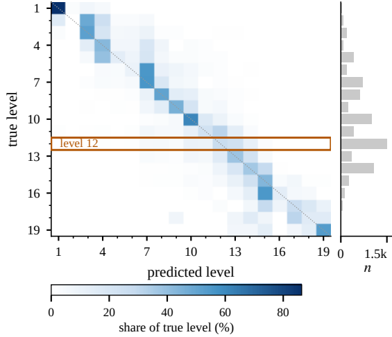
Figure 3: Official Strict system on dev: row-normalized confusion over the 19 levels, with per-level support n . The modal level 12 (orange) is systematically under-predicted toward the center; most of its mass lands on predicted levels 10–14 (§5.3).
