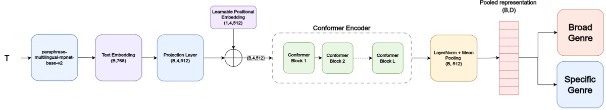
Figure 2: Core architecture of the proposed hierarchical genre classification model. The pretrained multilingual MPNet encoder produces a 768-dimensional text embedding, which is projected into four 512-dimensional representations, combined with learnable positional embeddings, processed by a stack of Conformer blocks, and pooled to generate broad- and specific-genre predictions.
