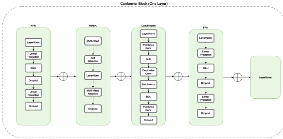
Figure 3: Internal architecture of a Conformer block used in the proposed projection module. Each block contains two feed-forward modules, a multi-head self-attention module, and a convolution module connected through residual connections, followed by a final LayerNorm operation.
