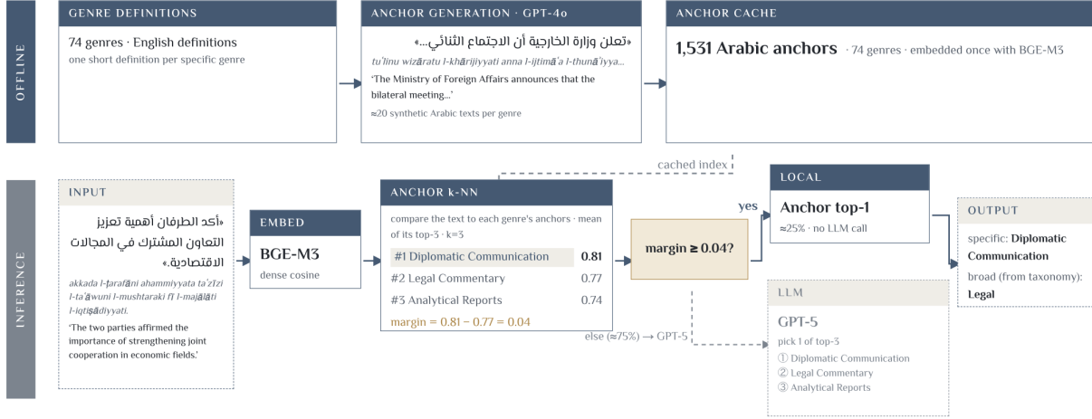
Figure 1: SynAnchor flat pipeline: offline anchor synthesis and margin-gated BGE-M3 retrieval with selective GPT-5 adjudication.
