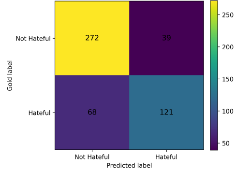
Figure 2: Development-set confusion matrix for the final late-fusion system.
