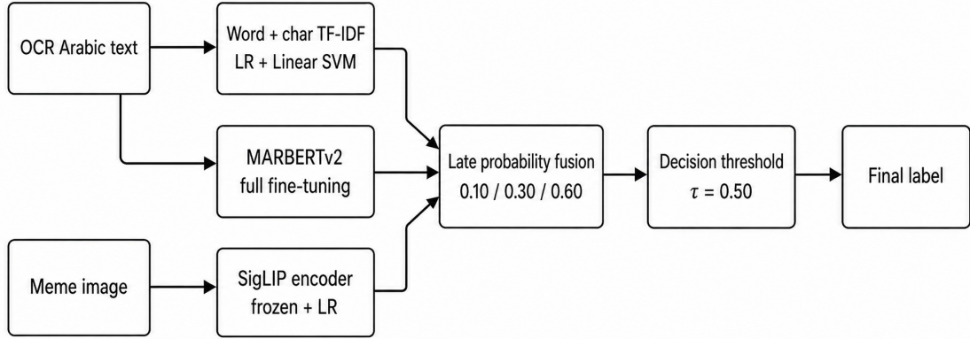
Figure 1: Architecture of the proposed late-fusion system.
