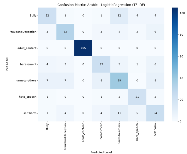
Figure 1: Confusion matrix for the Arabic Logistic Regression classifier on B2 development data.
