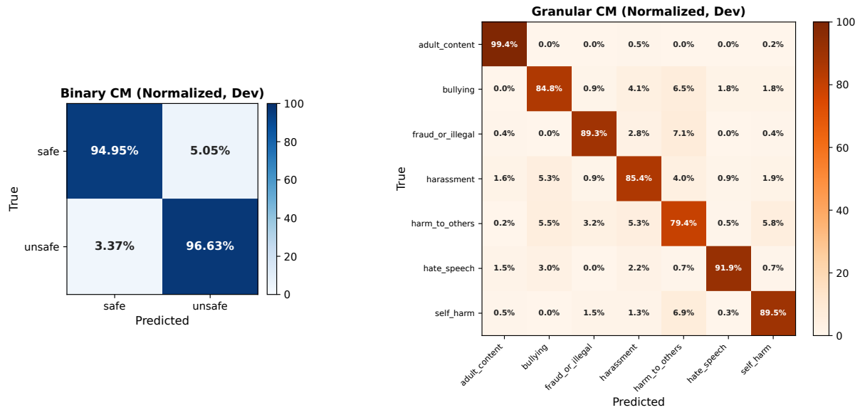
Figure 3: Row-normalized confusion matrices on the labeled development set. Left: binary classification; right: seven-way granular classification.
