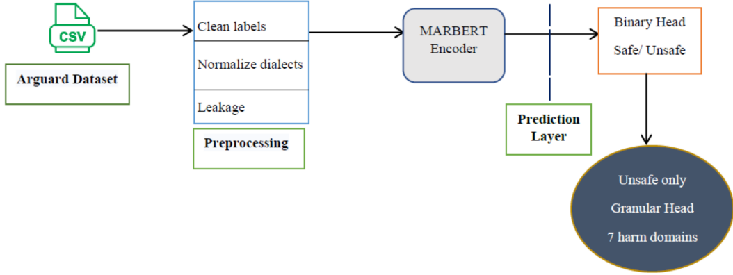
Figure 2: Overview of the multi-task classification system.
