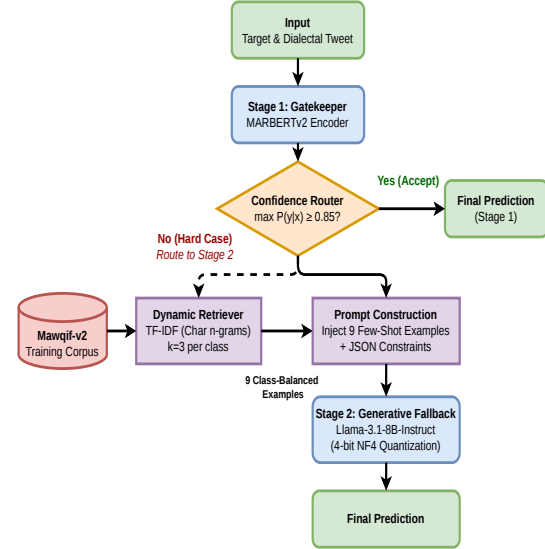
Figure 1: Architecture of the Two-Stage Hybrid Cascade. The MARBERTv2 gatekeeper rapidly classifies high-confidence tweets, while uncertain cases ( \tau < 0.85 ) are routed to a retrieval-augmented LLM.
