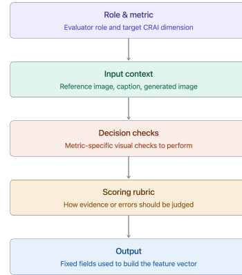
Figure 1: Prompt structure used for CRAI evaluation.
