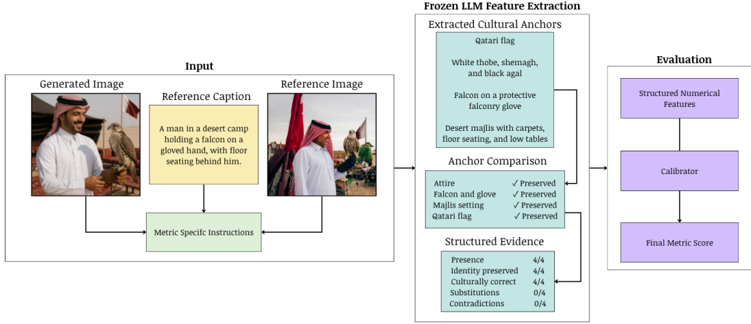
Figure 2: Overview of the proposed reference-based evaluation framework. Cultural anchors are identified from the reference image and caption, compared with the generated image to assess preservation, substitution, and cultural correctness, and then converted into numerical features for final score prediction.
