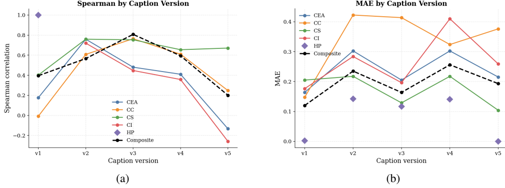
Figure 3: Performance across caption versions on the development set: (a) Spearman correlation and (b) MAE for the five CRAI dimensions and the composite score.
