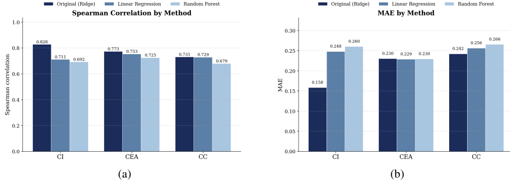
Figure 4: Comparison of the original score mapping with Linear Regression and Random Forest for CI, CEA, and CC: (a) Spearman correlation and (b) MAE on the development set.
