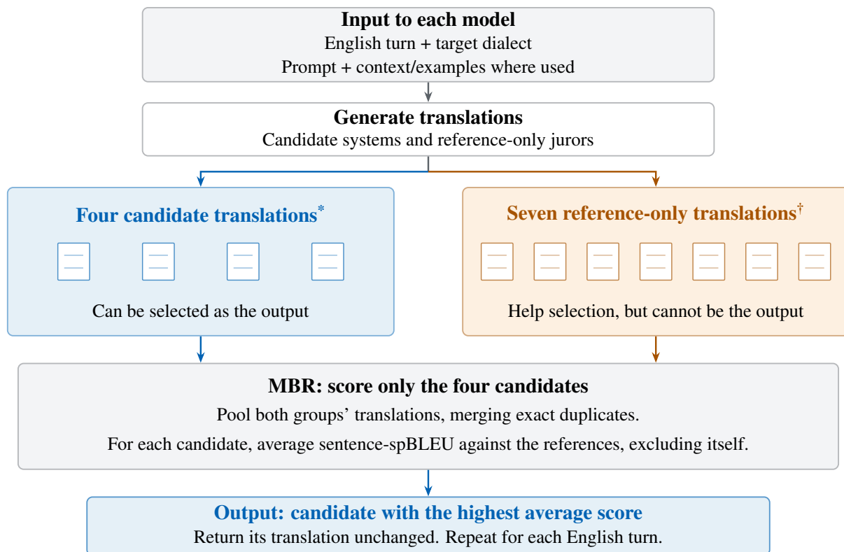
Figure 1: Candidate-constrained MBR: additional translations help choose the answer, but only a candidate can supply it. For each turn, we select the candidate with the highest average sentence-spBLEU against the other unique translations (Eq. 1). *Candidate models and training recipes: Table 2. †Reference-only jury models and prompts: Appendix A. The submitted system reaches 33.4891 macro spBLEU, 1.2554 above the best single candidate system and 0.8145 above choosing the best whole system separately for each dialect (32.6746). This retrospective comparator uses blind-test scores to choose one system for all turns in each dialect; MBR selects separately for each turn without hidden references (Section 2.2).
