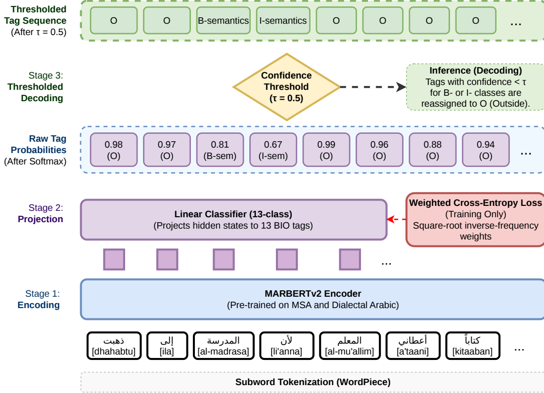
Figure 1: Architecture of our confidence-thresholded BIO token classification pipeline for joint MT error detection and classification.
