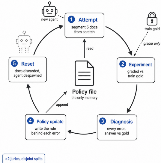
Figure 1: The jury training loop (Section 3). In each batch the jury reads its policy file, segments five training documents from scratch, is graded against the training gold, sees every error beside the annotator’s answer, and writes the rule behind each error into the file. The documents are then discarded and the agent is periodically replaced by a fresh one that receives only the policy file, which is the sole memory carried across batches; the gold is visible to the grader only. Two juries are trained this way for each track pair.
