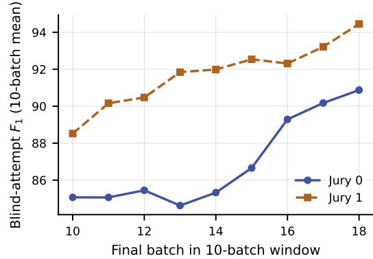
Figure 3: Blind-attempt F_1 of the two NoPnx-PA juries during training, averaged over a moving window of 10 batches (50 documents), in curriculum order. Each attempt is scored before the gold for its batch is revealed and no document is seen twice, so the curve reflects performance on unseen documents as the policy files grow. The juries train on disjoint halves of the corpus; NoPnx-PA is the track whose full training run is banked end to end, and the other tracks’ attempts are not recoverable in curriculum order.
