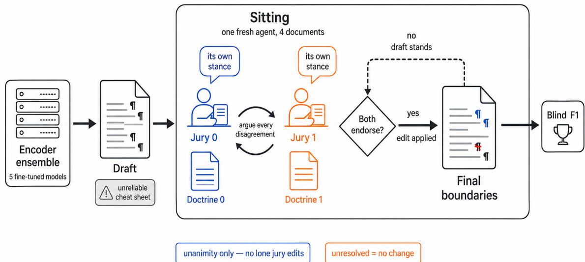
Figure 2: Adjudication at inference (Section 3). The encoder ensemble (five fine-tuned voters; a tuned three-voter subset for the Pnx-PA submission) produces a draft segmentation, which enters a sitting: one fresh agent holding four documents and both learned doctrines, treating the draft as an unreliable cheat sheet. Jury 0 and Jury 1 each state a stance from their own doctrine and argue every disagreement; an edit is applied only when both endorse it, and an unresolved site leaves the draft unchanged. The final boundaries are scored with the organizers’ script.
