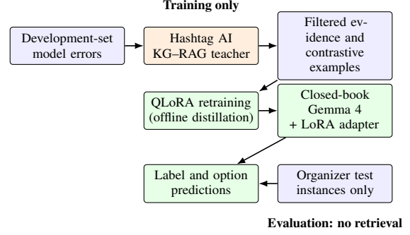
Figure 1: Knowledge-graph evidence is used only to construct and distill offline supervision. The submitted model receives no KG, retrieved evidence, search results, or external API access at evaluation time.
