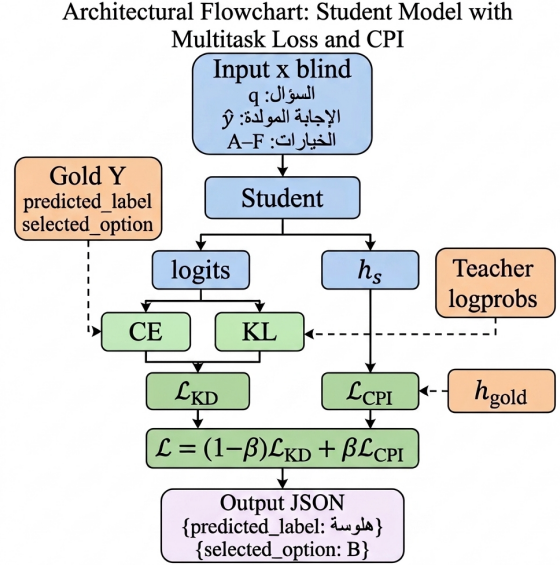
Figure 1: Overview of the Student training pipeline with Multitask Knowledge Distillation ( \mathcal{L}_{\text{KD}} ) and Contrastive Privileged Information Alignment ( \mathcal{L}_{\text{CPI}} ) for Arabic hallucination detection.
