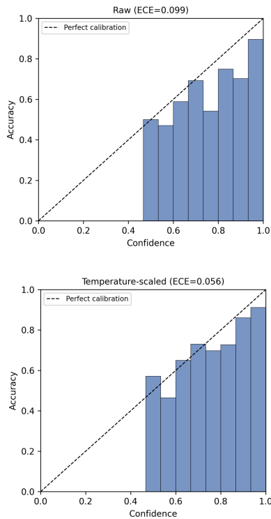
Figure 1: CAMELBERT reliability diagrams before and after temperature scaling.
