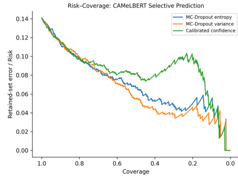
Figure 2: Selective risk-coverage for CAMELBERT. Lower retained-set risk is better as uncertain cases are deferred.
