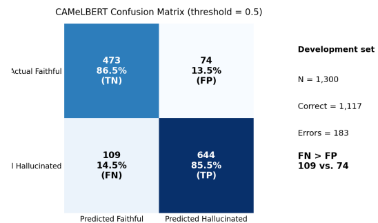
Figure 3: CAMELBERT development confusion matrix at threshold 0.5: 473 TN, 74 FP, 109 FN, and 644 TP. False negatives are more frequent than false positives at this operating point.
