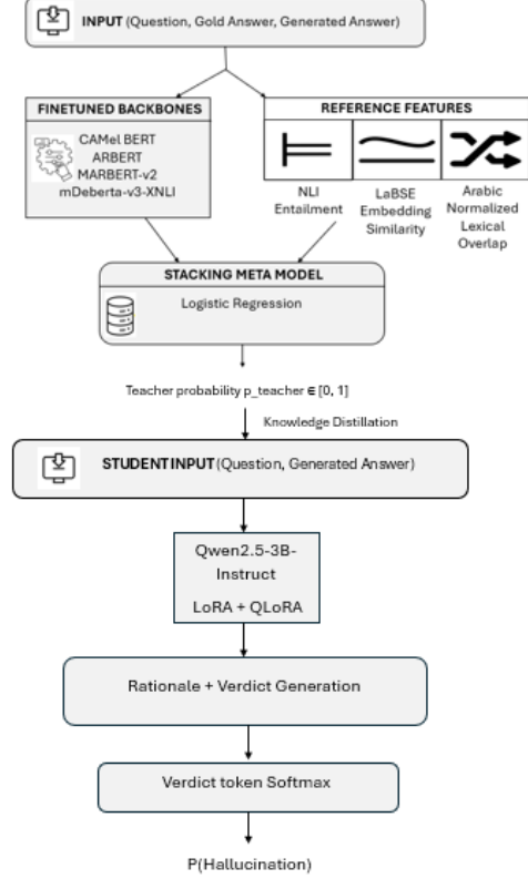
Figure 1: Overview of the Student-Teacher Model.
