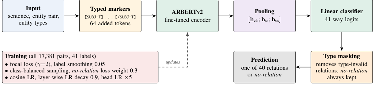
Figure 1: Our RE pipeline. Typed entity markers are inserted around the subject and object, the sentence is encoded by a single fine-tuned ARBERTv2 encoder, and the state of the classification token ([CLS]) is concatenated with the states at the subject and object start markers and classified into 41 labels (40 relations plus no-relation ). Training (bottom left) uses all pairs, including no-relation , with imbalance-aware objectives. At inference, ontology-based type masking removes relations whose domain or range is incompatible with the entity types; no-relation is never masked.
