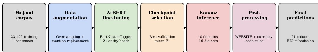
Figure 1: End-to-end system pipeline, from Wojood training data through augmentation, fine-tuning, checkpoint selection, Konooz inference, and post-processing to the final submission.
