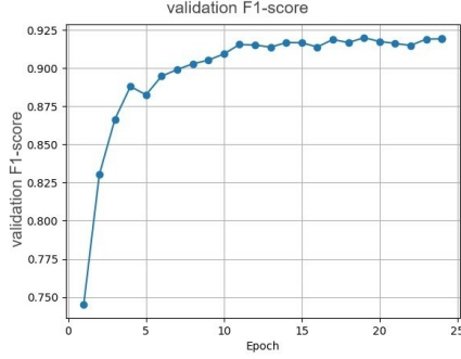
Figure 2: validation F1-score during training
