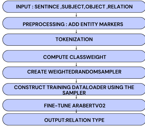
Figure 1: Overview of the submitted system
