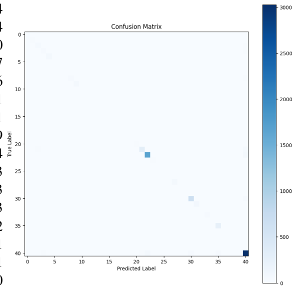
Figure 4: Confusion Matrix for validation dataset
