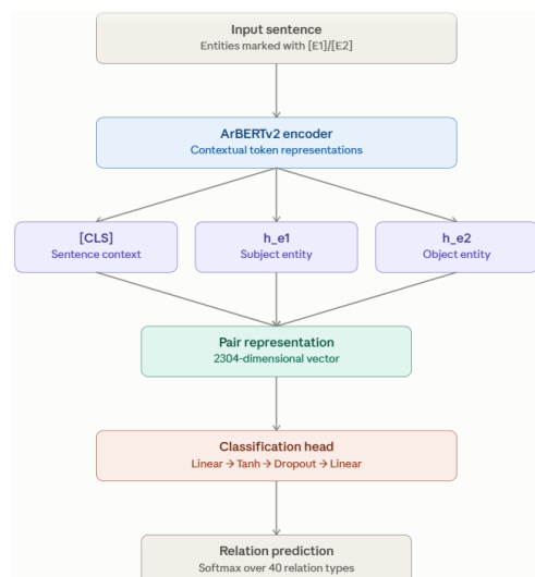
Figure 2: The ArBERTv2 entity-marker architecture used for the relation classification subtask.
