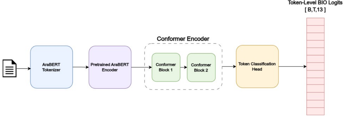
Figure 2: Overview of the proposed ADU detection pipeline. The system processes an Arabic paragraph using AraBERT tokenization, overlapping token windows, an AraBERT encoder, a Conformer tagging head, and a token-level classifier before reconstructing final character-level ADU spans.
