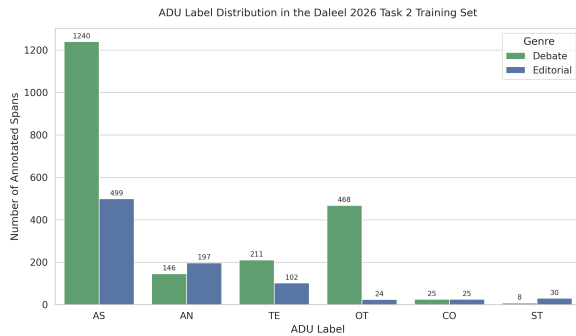
Figure 1: Distribution of ADU labels in the Daleel 2026 Task 2 training set across the two text genres: editorials and debates. The figure shows the strong class imbalance in the dataset, especially for CO and ST.
