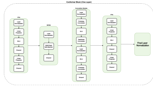
Figure 3: Structure of the Conformer block used in the tagging head. The block combines feed-forward layers, multi-head self-attention, and a convolution module to capture both global contextual information and local span-boundary cues.
