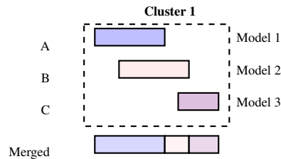
Figure 1: Example of character-level span clustering given 3 sets of predicted spans extracted from the same paragraph. Overlapping spans form a connected cluster and are merged using the minimum start and maximum end offsets.
