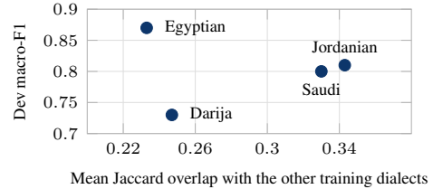
Figure 3: Per-dialect dev macro-F1 (single seed) against lexical distance (mean Jaccard overlap in Figure 1): the two most distinct dialects are the easiest and the hardest.
