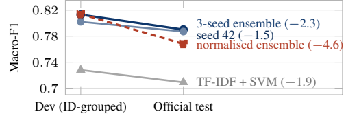
Figure 2: Dev-to-test generalisation of the four submitted systems (Table 1): raw-text systems lose 1.5 to 2.3 points, whereas the normalised ensemble loses 4.6.
