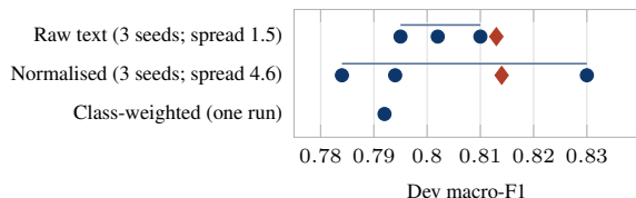
Figure 4: Seed variance versus interventions on dev: single runs (dots) span 1.5 points for raw text, normalisation widens the spread to 4.6, and the two ensembles (diamonds) are indistinguishable.
