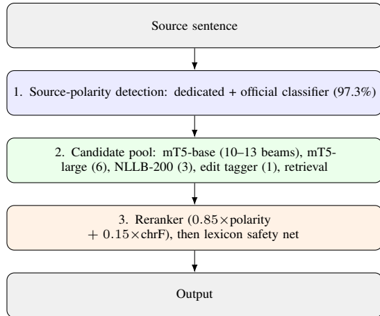
Figure 1: Inference pipeline. Retrieved near-duplicates are ordinary candidates, not a bypass, and four generators feed a single reranker.
