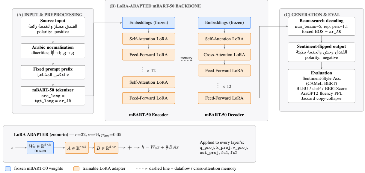
Figure 1: Overall system architecture. (A) Source dialectal Arabic text is normalised (diacritics stripped; alef/yaa/hamza variants canonicalised) and wrapped in a fixed اعكس المشاعر prefix before being tokenised by the mBART-50 tokenizer with both source and target languages set to ar_AR . (B) The tokenised sequence is consumed by a frozen mBART-50 encoder-decoder ( \approx 610 M parameters); low-rank LoRA adapters are attached to every attention and feed-forward projection ( q_proj , k_proj , v_proj , out_proj , fc1 , fc2 ). (C) At inference, beam search with forced_bos_token_id set to ar_AR produces the sentiment-flipped Arabic sentence, which is scored with the official Sentiment-Style Accuracy metric alongside BLEU, chrF, BERTScore, an external AraGPT2 fluency perplexity, and our Jaccard copy-collapse diagnostic. The bottom inset details a single LoRA adapter: only the low-rank factors A and B are trained ( r=32 , \alpha=64 ), while the base projection W_0 remains frozen.
