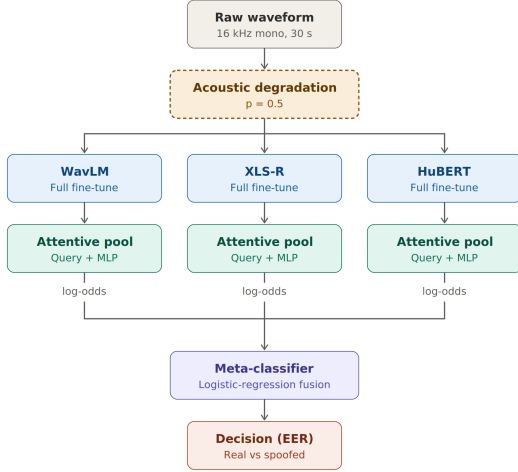
Figure 1: Overview of the proposed system. The raw waveform is first passed through the acoustic degradation pipeline, drawn with a dashed outline to indicate that it is applied stochastically with probability p = 0.5 . The (optionally degraded) waveform then feeds three fine-tuned self-supervised encoders, each with an attentive-pooling head. The resulting bonafide log-odds are fused by a logistic-regression meta-classifier to produce the real-vs-spoofed decision.
