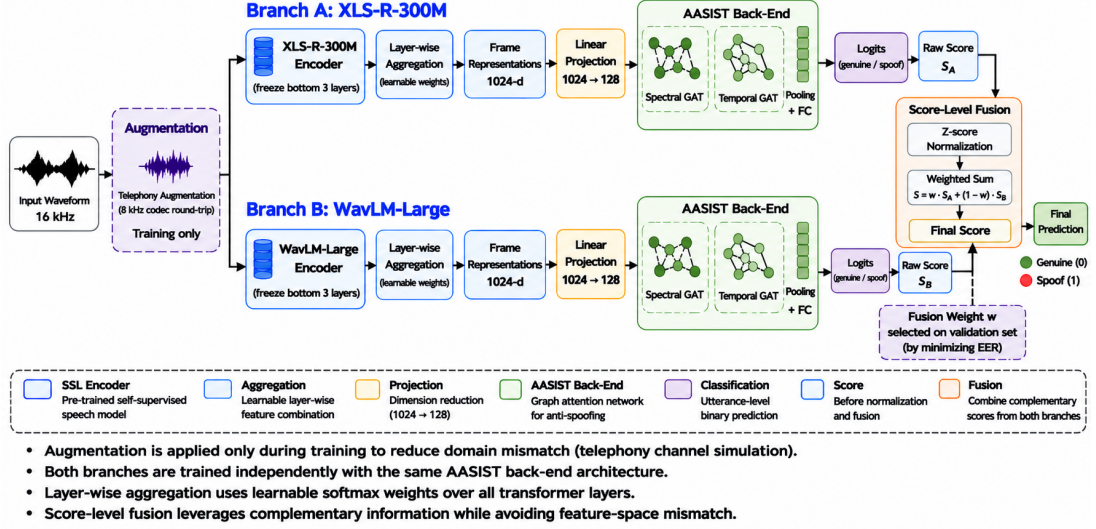
Figure 1: Proposed dual-branch SSL+AASIST architecture with weighted score-level fusion.
