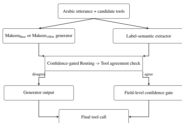
Figure 7: Overview of the Makeeen pipeline. The submitted Makeen Base generator is extended with label-semantic extraction for Makeen +Hint and with confidence-gated routing at inference time.
