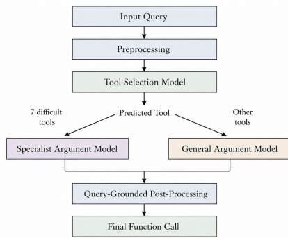
Figure 1: Overview of the ArgTune modular architecture.
