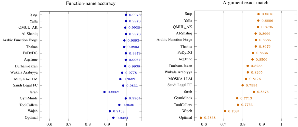
Figure 2: Component scores for all 17 Track A systems in official rank order. The panels share the same horizontal range. High function-name accuracy must be interpreted in light of the input shortcuts in Section 7.1.
