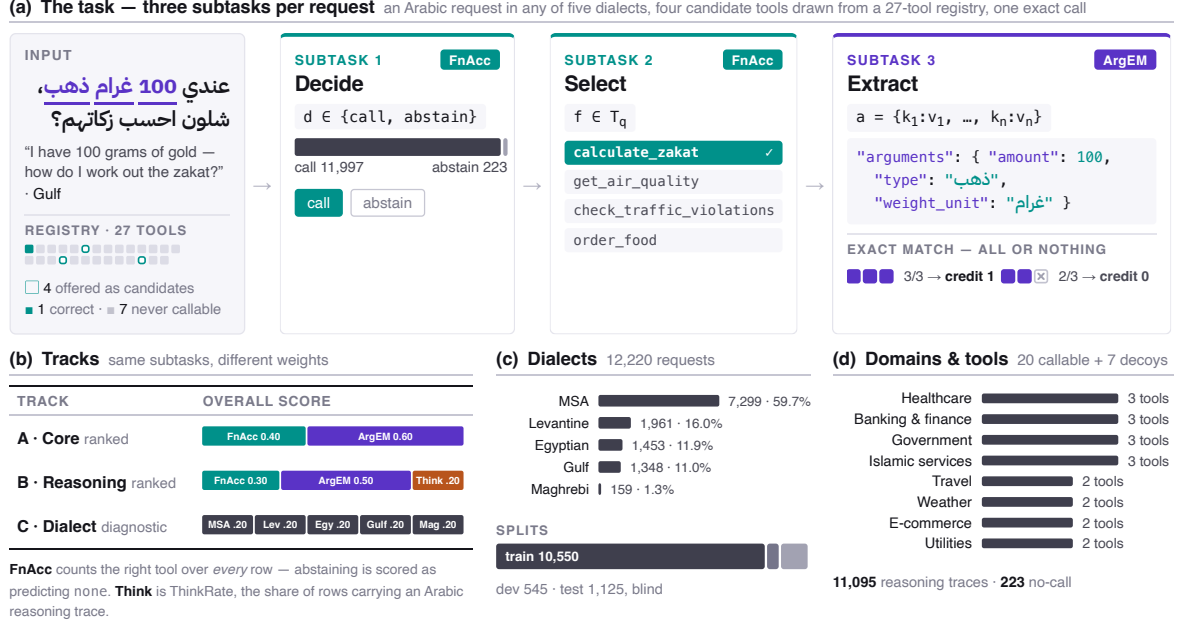
Figure 1: Overview of the AISA-ArabicFC shared task. Each request requires either one structured function call or abstention. Tracks A and B evaluate submitted predictions; Track C provides a dialect-level diagnostic.
