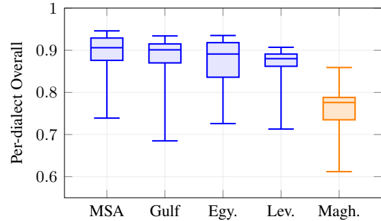
Figure 3: Per-dialect Overall scores across the 21 Track C systems. Boxes show the interquartile range, internal lines show medians, and whiskers show minima and maxima. Maghrebi has the lowest score for every system; its maximum (0.859) is below the median of each other dialect group.
