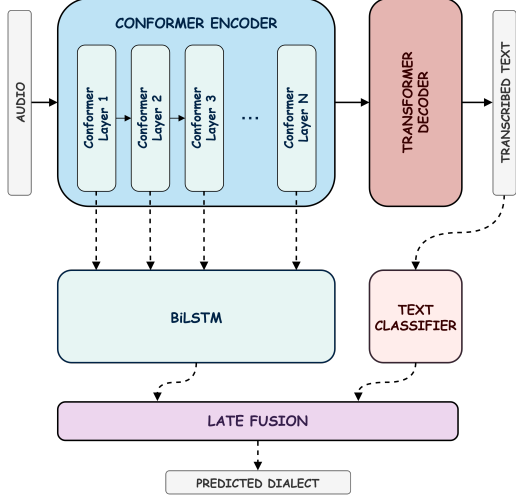
Figure 1: Overview of the Lynx_Id architecture for spoken dialect identification.
