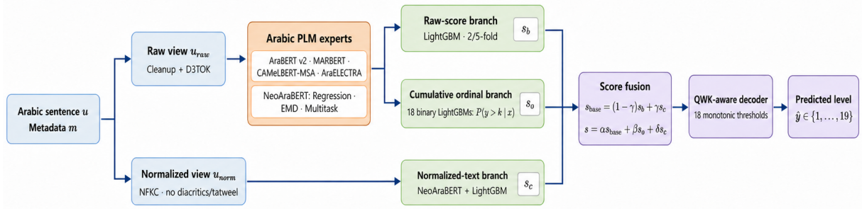
Figure 1: Sentence-level architecture. The raw Arabic sentence is processed by the PLM feature path, whereas a normalized text view is used by a complementary normalized-text branch. A stricter normalized key is used only for a training-only exact lookup. The three branches output continuous difficulty scores, which are fused and decoded into one of 19 ordered levels.
