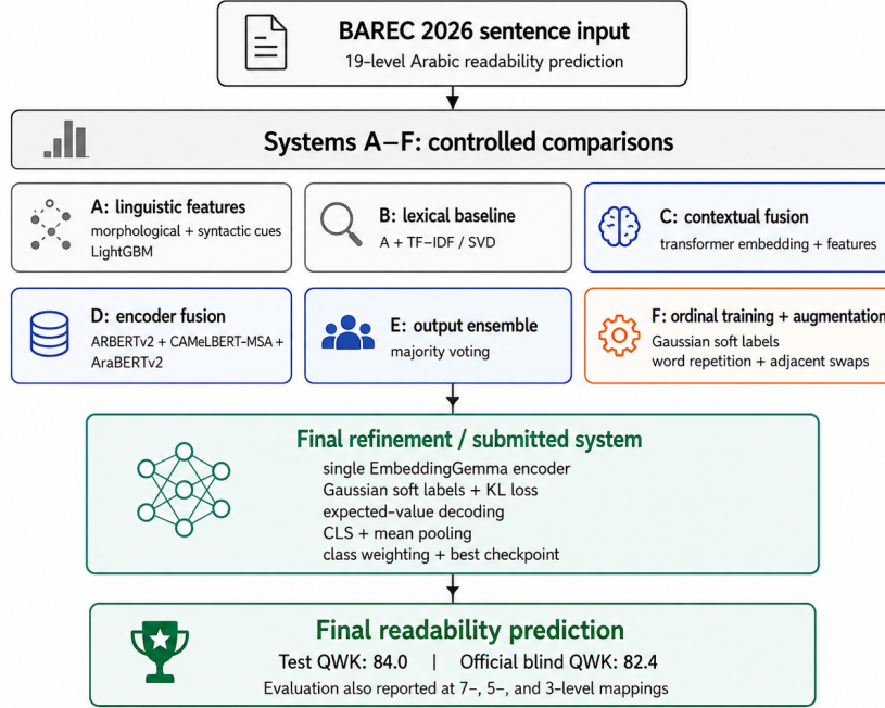
Figure 1: Overview of the BAREC 2026 system progression. Systems A–F provide controlled comparisons from linguistic and lexical baselines to contextual, multi-encoder, ensemble, and ordinal-aware configurations.
