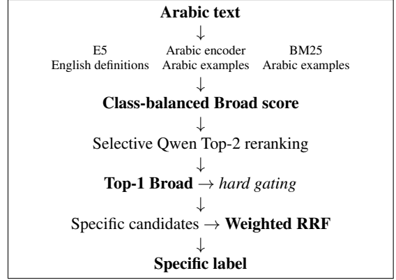
Figure 1: Final class-balanced hierarchical retrieval pipeline.
