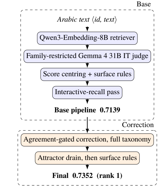
Figure 1: System overview. A Qwen3 retriever gates a broad family and a Gemma 4 31B IT judge scores its siblings setwise; score centring, surface rules and a binary Interactive-recall pass complete the five-step base pipeline (0.7139). GPT 5.6 Luna and Gemini 3.6 Flash, shown all 74 definitions, then change a label only where they agree, and an attractor drain follows (0.7352, rank 1).
