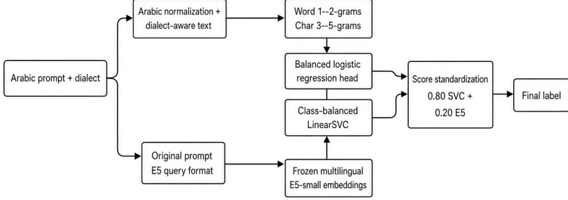
Figure 1: Architecture of the proposed hybrid Arabic prompt-safety classification system
