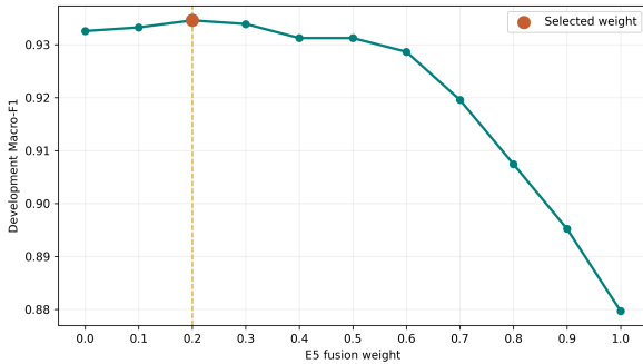
Figure 2: Development Macro-F1 across E5 fusion weights
