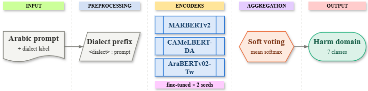
Figure 1: System overview. The dialect tag is prepended to the prompt; three Arabic encoders with complementary pre-training corpora are each fine-tuned under two seeds, and the six softmax distributions are averaged.
