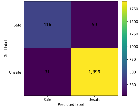
Figure 3: Development confusion matrix for the final sparse fusion system.
