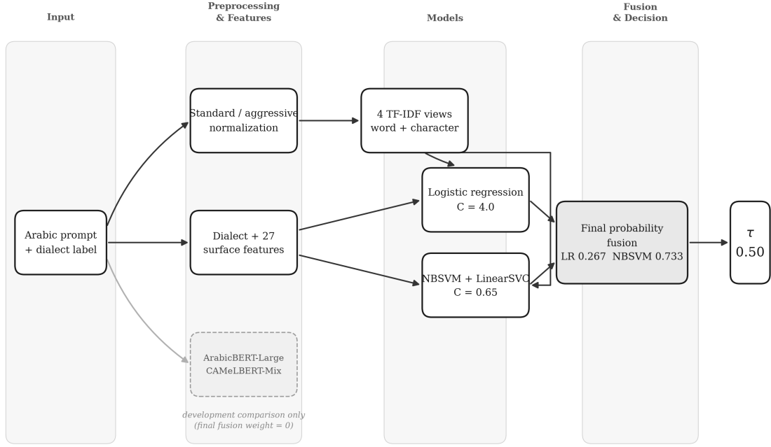
Figure 1: Architecture of the Arabic dialect-aware classification system
