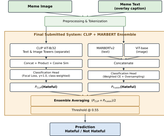
Figure 1: Workflow of the final CLIP-MARBERT ensemble system.
